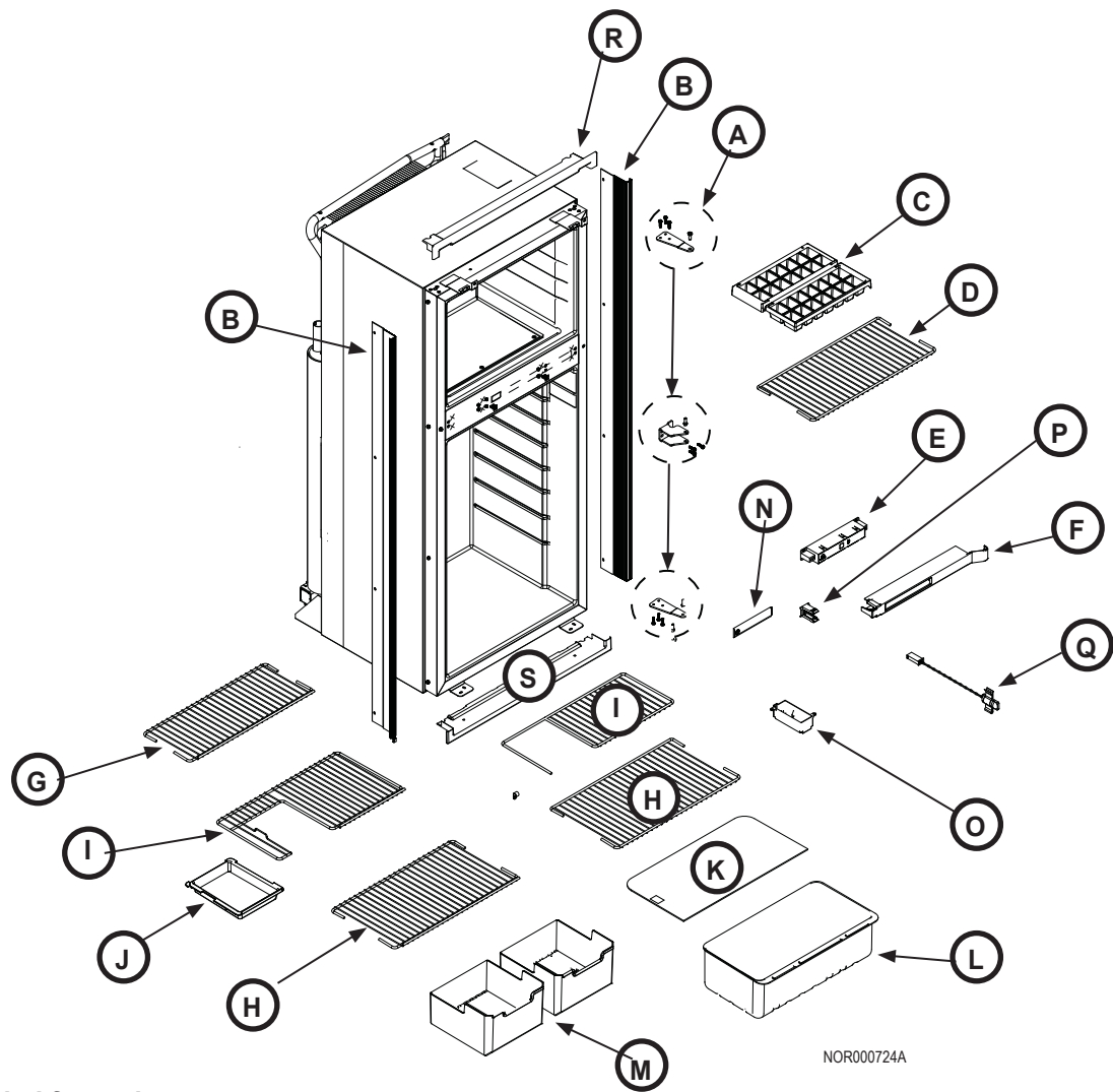
Fig. 4 - Exploded front view
