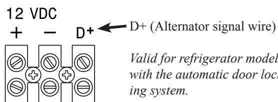
FIG 18 - ALTERNATOR CONNECTION
